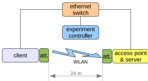
Fig. 1. Schematic of test-bed showing physical connectivity. The testbed was configured separately for experiments with 802.11g (2.4GHz) and 802.11n (5GHz, 20MHz channels). The experiment controller uses Ethernet for control messages and shared file-system access. The separation between the antennas of the client and access point/server is 24m, attenuators (att.) and transmission power control were used to adapt the signal strength. Data packets generated by iperf were transferred across the WLAN.
