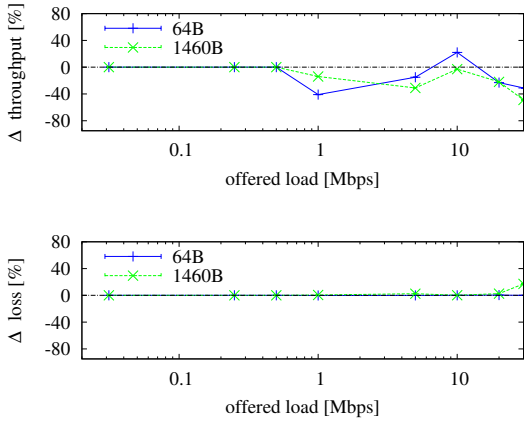
Fig. 3. Differences in throughput and loss of IEEE 802.11g between and IEEE 802.11n with low ( \sim 85 dBm) RSSI. Horizontal zero line is a visual aid. Positive values indicate where 11g has higher values.
